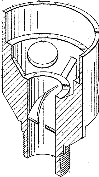
1.1 PERSPECTIVE VIEW
