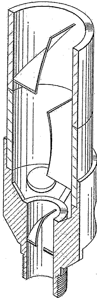
1.1 PERSPECTIVE VIEW
